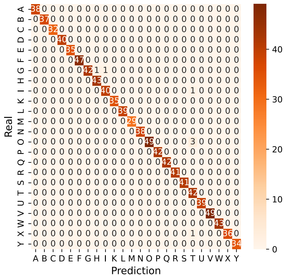
Fold 3
