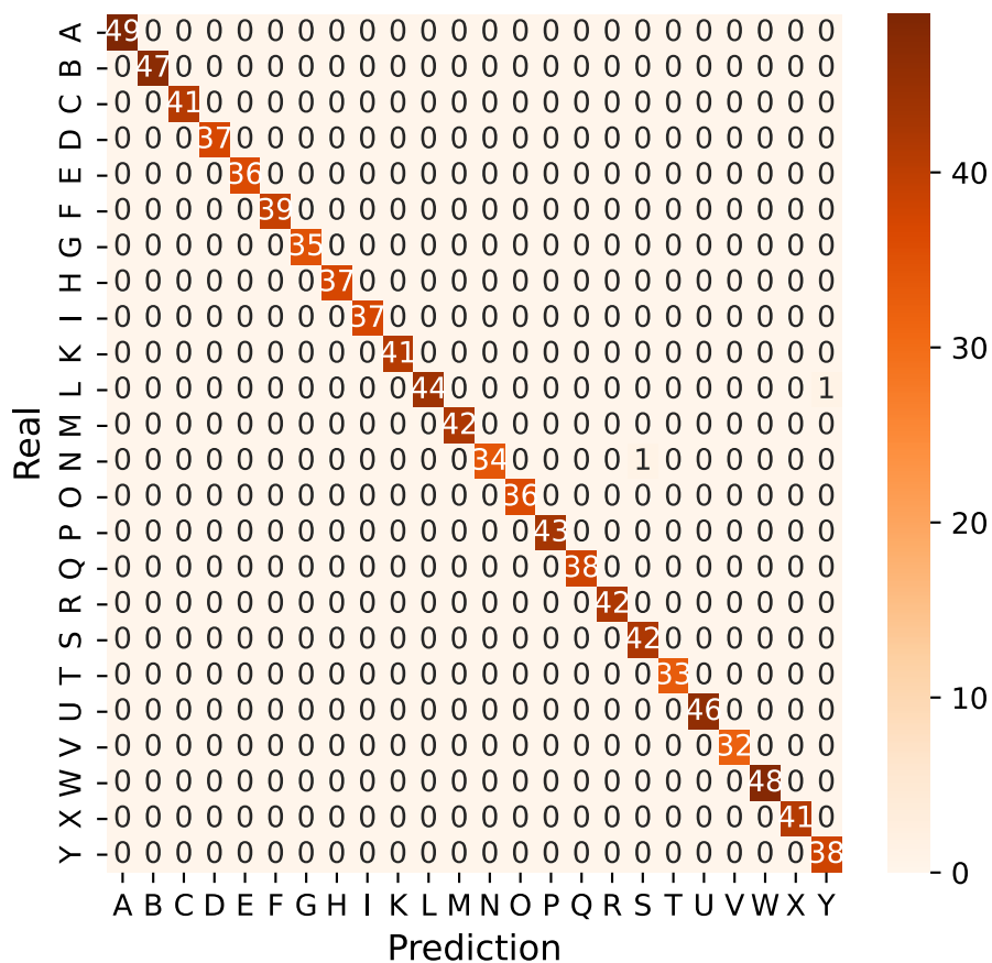
Fold 4
